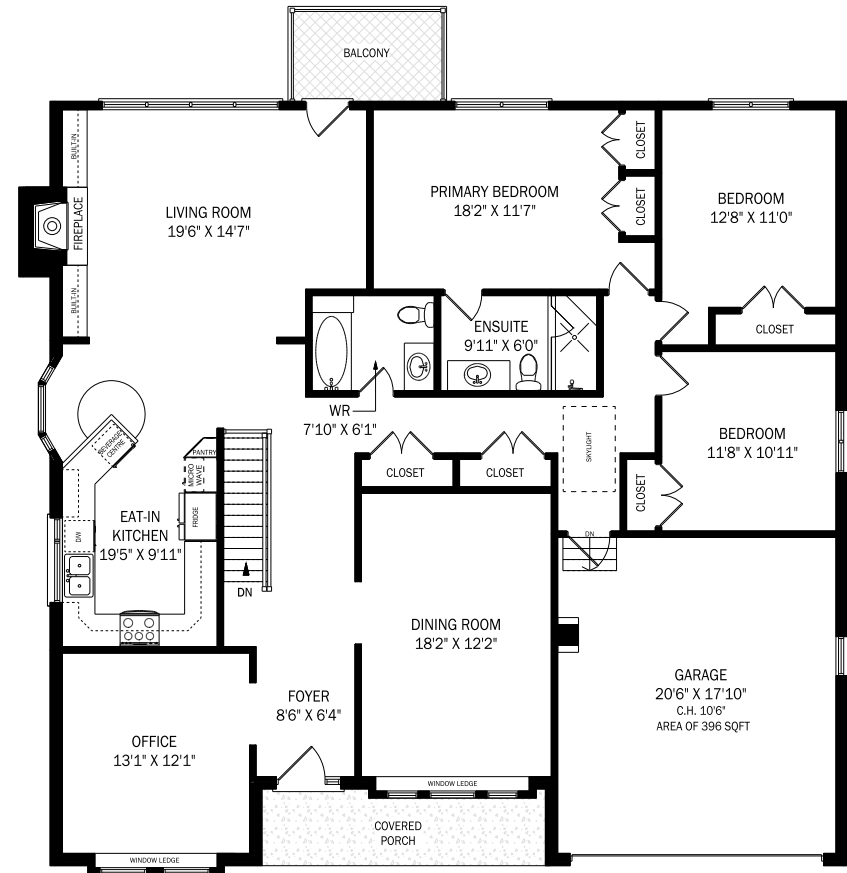
CEILING HEIGHT 8'0" MAIN FLOOR - 2036 SQUARE FEET
