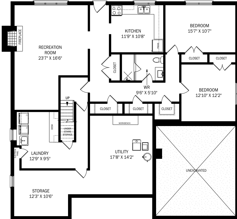
LOWER LEVEL - 2022 SQUARE FEET
